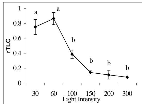
Figure 9. Relative total lipid content (rTLC) under various light intensities (n=3). Different letters indicate significant difference (P<0.05). Error bar represents standard error (n=3)
