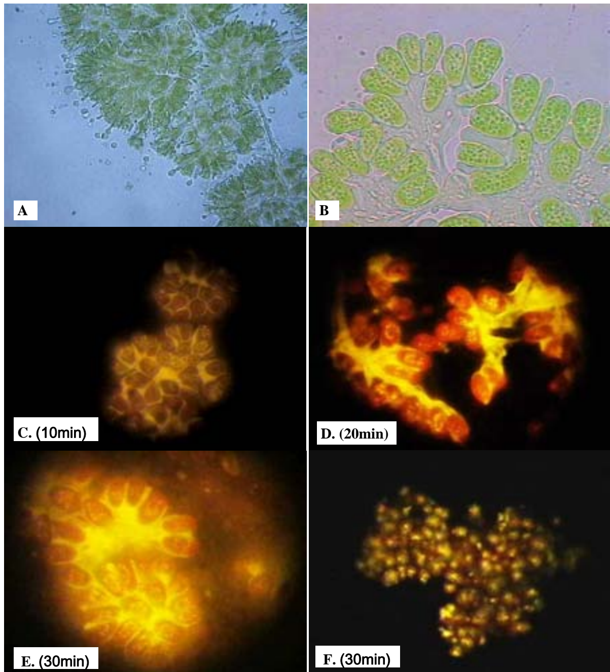
Figure 2. The algal microstructure of B. braunii (China strain 2). (A— Cells are embedded in a gelatinous mass containing oil drops extruded from the extracellular pool by pressing; B— there are many oil particles in the algal cells, including nucleus; C— the fluorescence picture of algal cells after 10 min staining. The reddish staining colour is chlorophylls and the yellow colour is lipid after staining; D— the intercellular and extracellular lipid fluorescence become obvious after 20 min staining; E— the lipid fluorescence of algal cells is stronger after 30 min staining; F— the fluorescence picture of an algal colony after 30 min staining)
