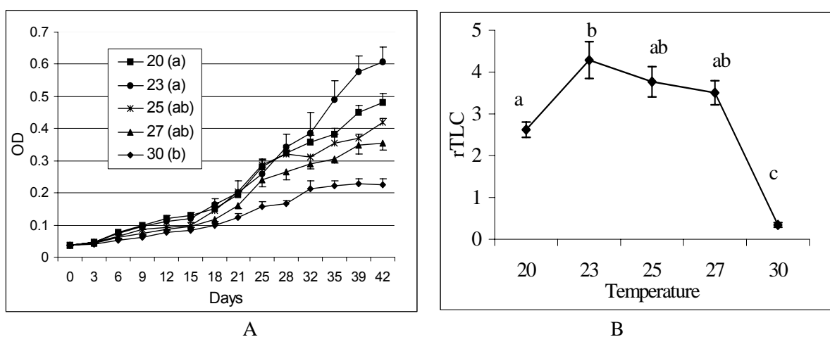
Figure 6. A: The impact of temperature on algal growth over time, and B: the impact of temperature on lipid production (rTLC). Error bar represents standard error (n = 4). Different letters indicate significant difference ( P < 0.05 ).
