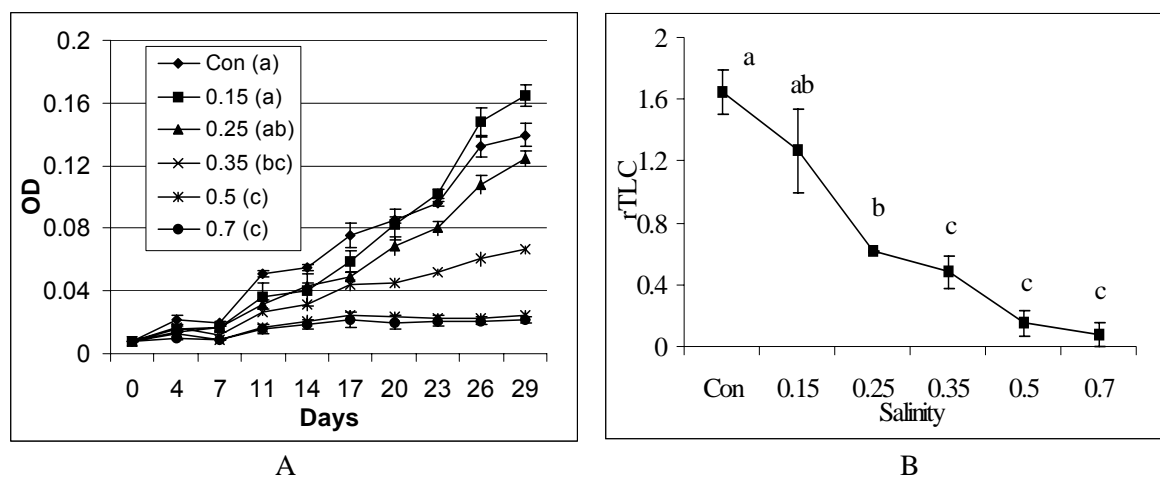
Figure 10. The impact of salinity on the algal growth over time (A); and the mean lipid production (rTLC) of B. braunii at different salinities (B). Different letters indicate significant treatment difference ( P < 0.05 ). Error bar represents standard error ( n = 3 ).
