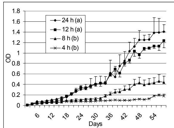
Figure 5. Impact of different photoperiods on algal growth. Different letters indicate significant difference ( P < 0.05 ). Error bar represents standard error ( n = 3 ).
