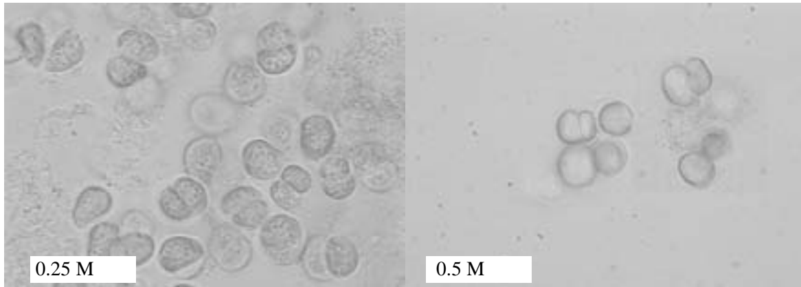
Figure 11. The morphology of algal cells in 0.25 and 0.5 M NaCl.
