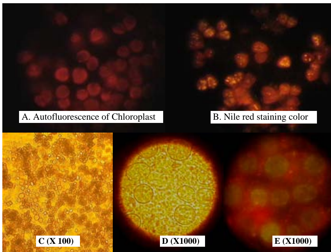
Figure 3. Illustration of China strain 1. (A— Chloroplast autofluorescence without Nile red staining; B— With Nile red staining, the intracellular oil particles display yellow fluorescence and chloroplasts are reddish; C— The morphology of an algal colony, combined with many empty and round particles; D— The particle shape under mixture lights; E— Fluorescence of stained particles.)
