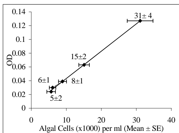
Figure 1. The relationship between OD and the amount of cell (ml).
