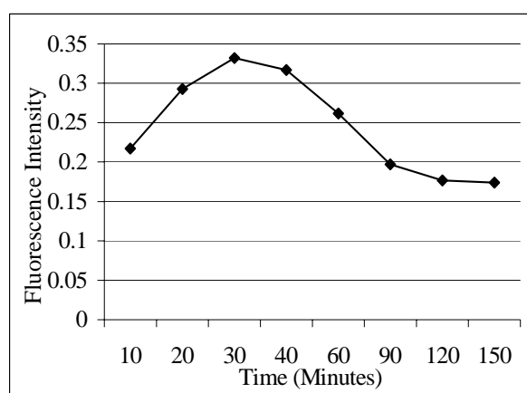
Figure 4. Fluorescence intensity at different reading time.
