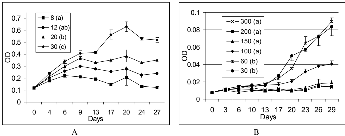
Figure 8. The impact of light intensity on algal growth. (A) Low light range; (B) High light range. Different letters indicate a significant treatment difference ( P < 0.05 ). Error bar represents standard error ( n = 3 )
