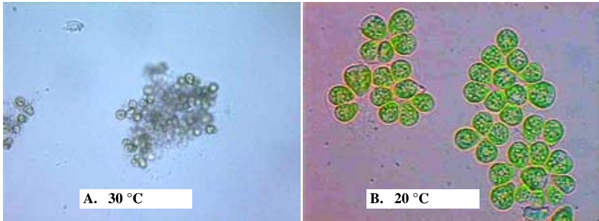
Figure 7. Morphological character of algal cells under 30 °C (A) and 20 °C (B).
